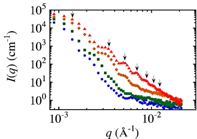
FIG. 2. (Color online) Azimuthally averaged scattering intensity, I , as a function of wave number, q , of dilute microgels described in Fig. 1 for the following temperatures: T = 24.6 (circles), 30.8 (squares), 32.6 (diamonds), and 34.7^\circ C (triangles). The scattering intensity decreases rapidly with q at lower temperatures. At the highest temperature, seven peaks or shoulders are clearly visible (arrows).
