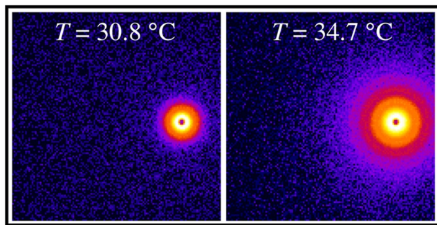
FIG. 1. (Color online) False color images of the small angle neutron scattering patterns from poly-NIPAM microgel particles at 1% by mass in a 9:1 mixture of D_2O:H_2O . Temperatures are: T = 30.8^\circ C < T_{lc} (left) and T = 34.7^\circ C > T_{lc} (right). The brighter and darker colors correspond to higher and lower intensities, respectively. The transmitted beam has been blocked (small dark inner circle), and the detector has been shifted out of the center to provide a greater range of scattering angles. Bright concentric rings around the beam block are observed to shift toward larger scattering angles as the temperature is increased.
